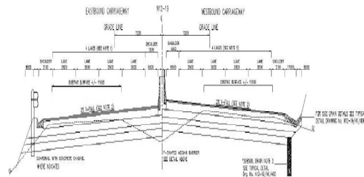
N12-19 TYPICAL 4 LANE CROSS SECTION
